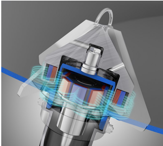
■ Figure 2 Principle of a radial magnet coupling.
